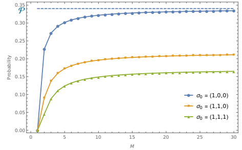
Fig. 6. Lower bounds obtained by PRISM on the termination probability of C_{3\text{dsrw}} in Exmp. 24 on initial position \sigma_0 . \mathcal{P} \approx 0.34 marks the true termination probability when starting from a neighbor location of the origin, e.g., \sigma_0 = (1, 0, 0) ; the true termination probabilities on other initial positions are unknown.
